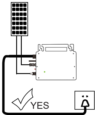
Connection diagram
